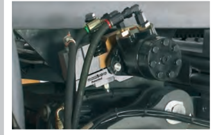
Hydraulic motor and brake (patented)
