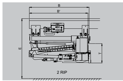
Side fitting for rigid vehicle - 2 folds platform
