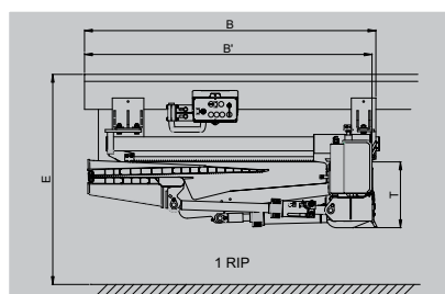
Side fitting for rigid vehicle - 1 fold platform
